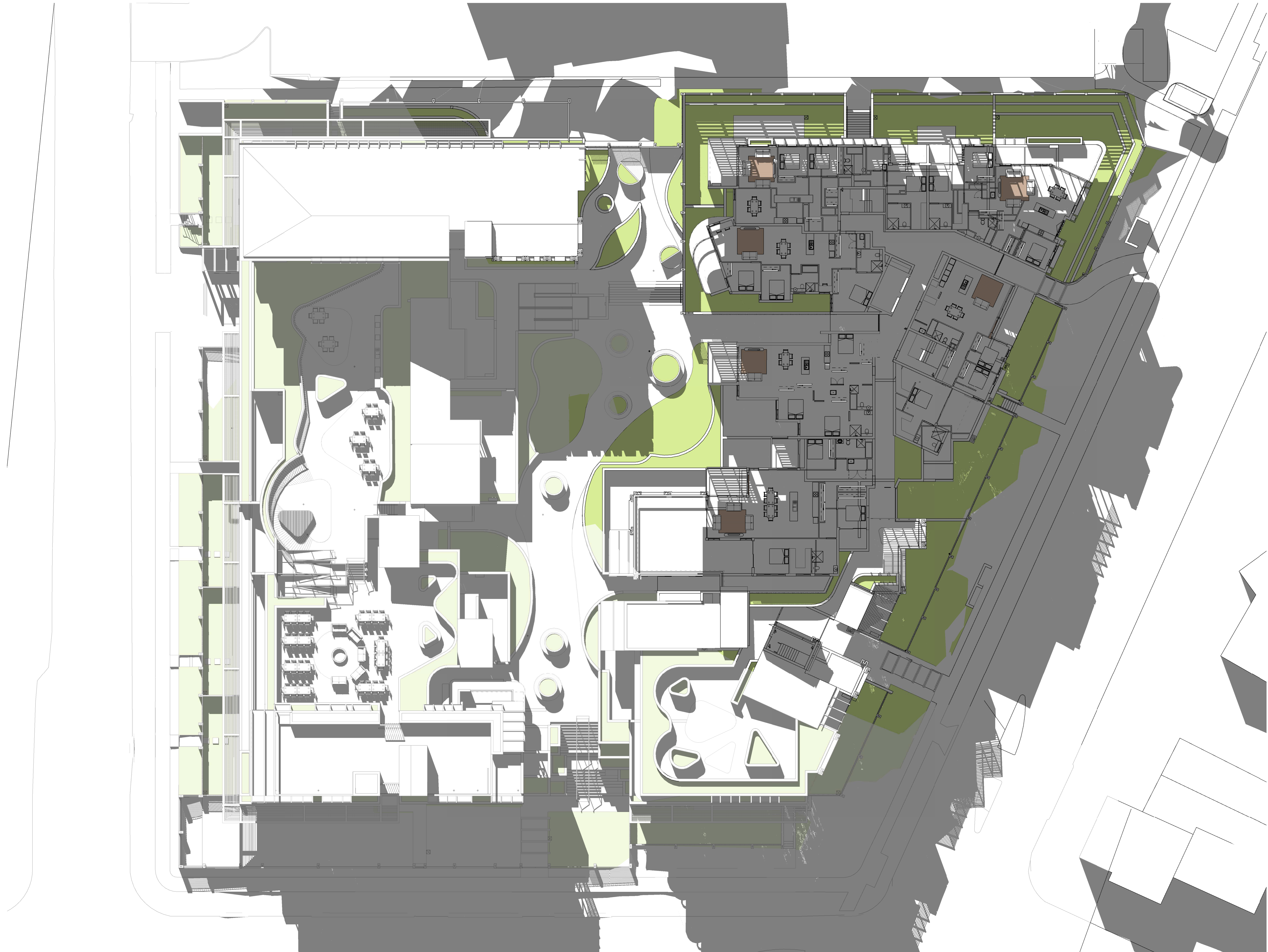
1 Internal Solar Access - Level 5 12pm June 21
