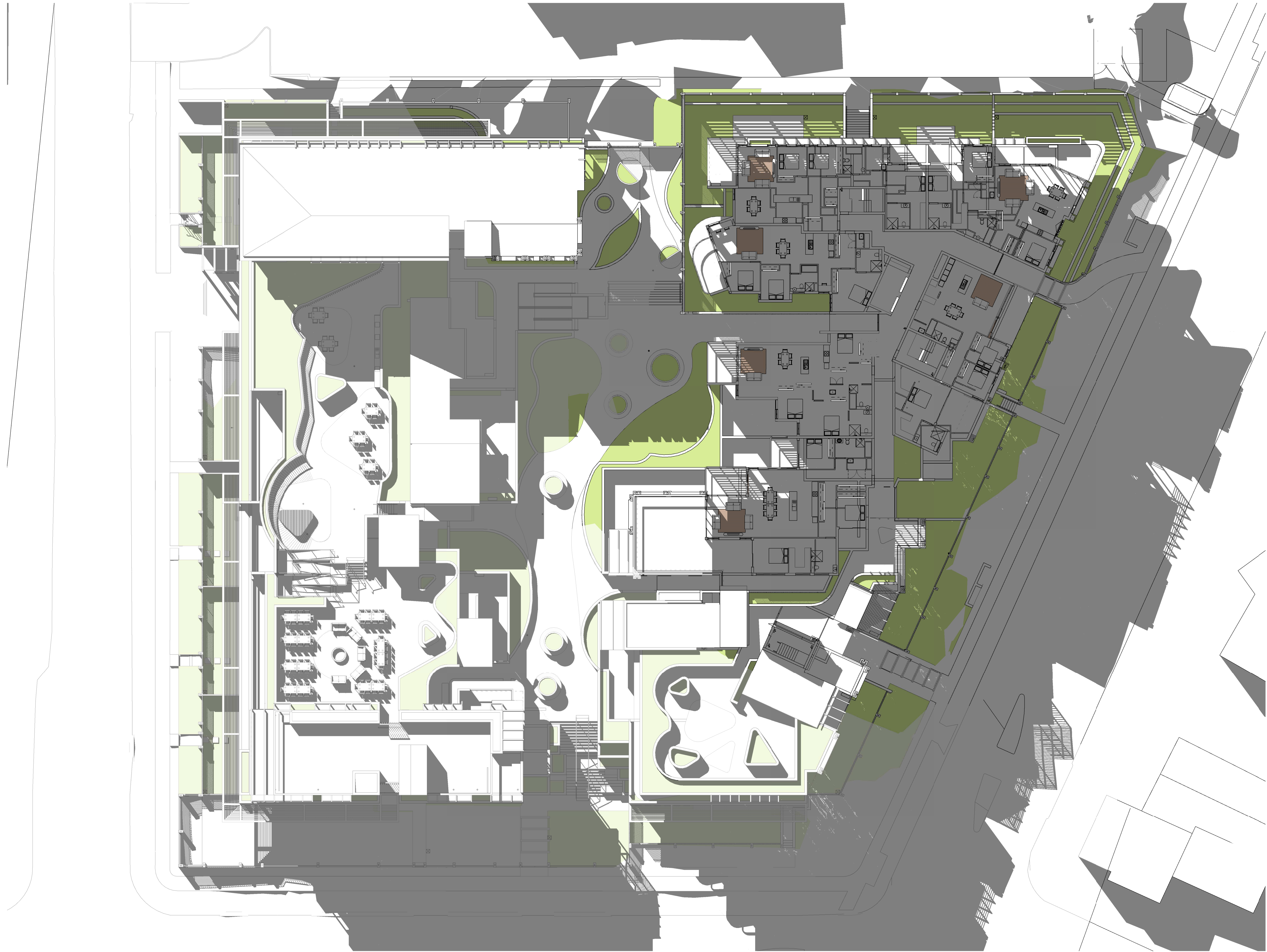
1 Internal Solar Access - Level 5 1pm June 21
