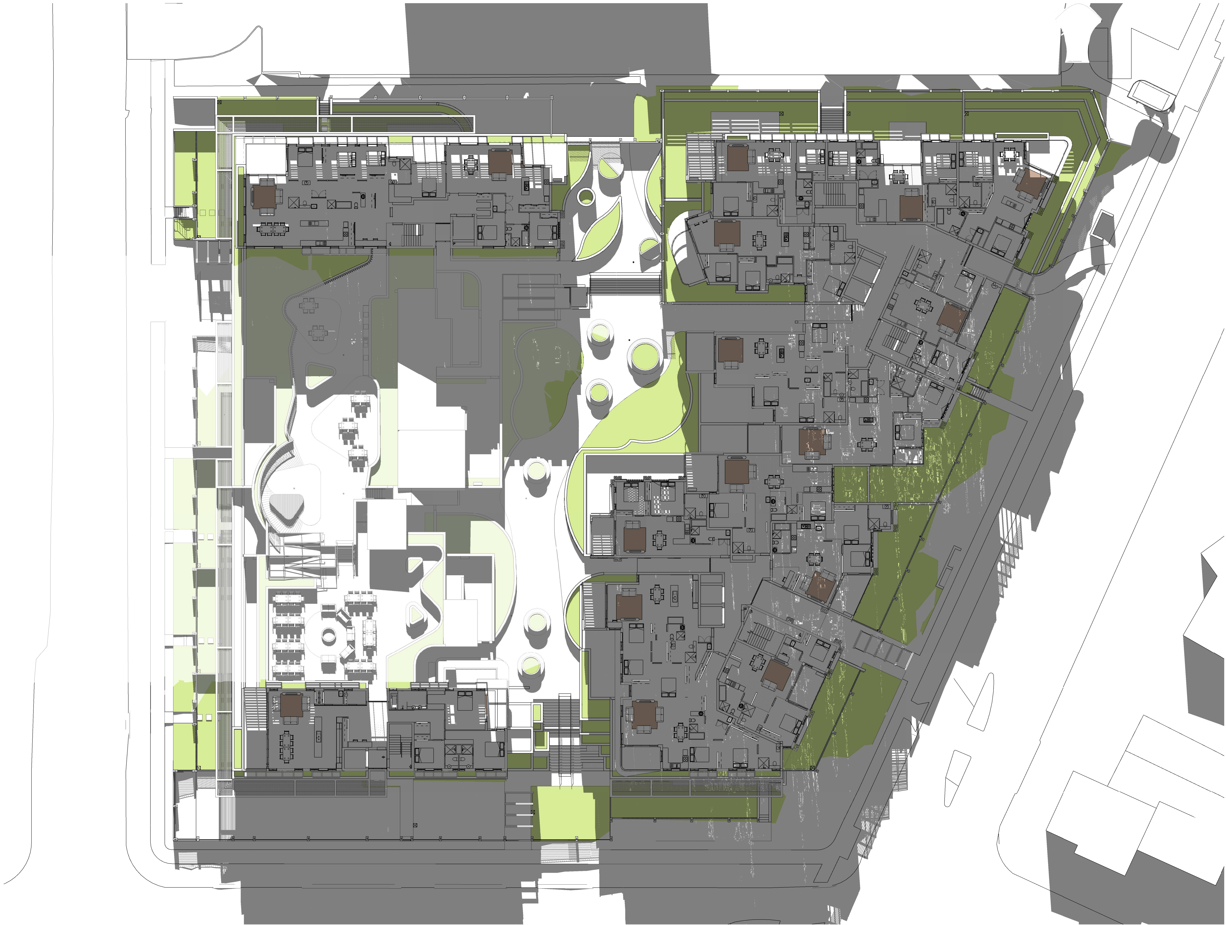
1 Internal Solar Access - Level 3 11am June 21
