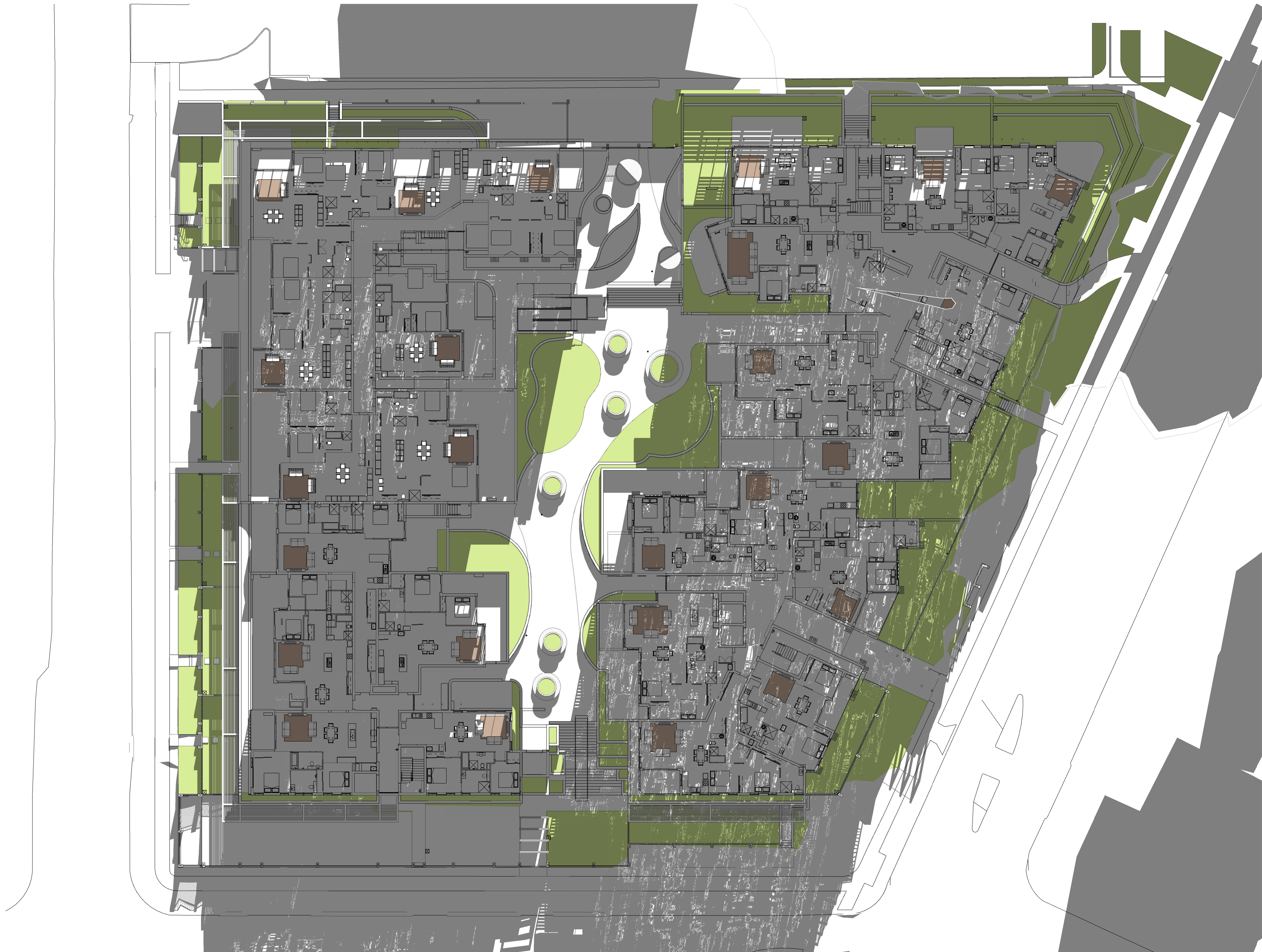
1 Internal Solar Access - Level 1 10am June 21
