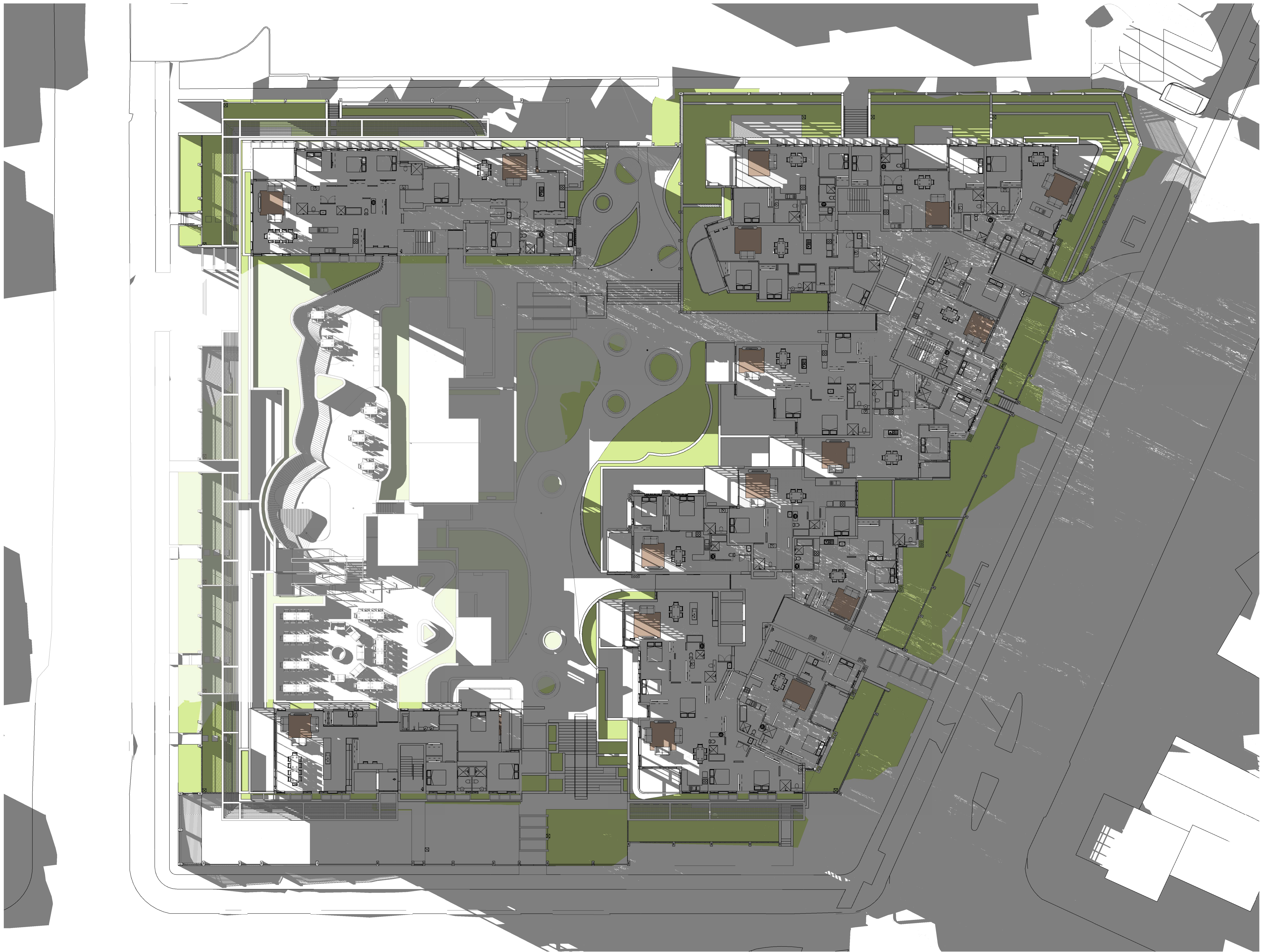
1 Internal Solar Access - Level 3 3pm June 21
