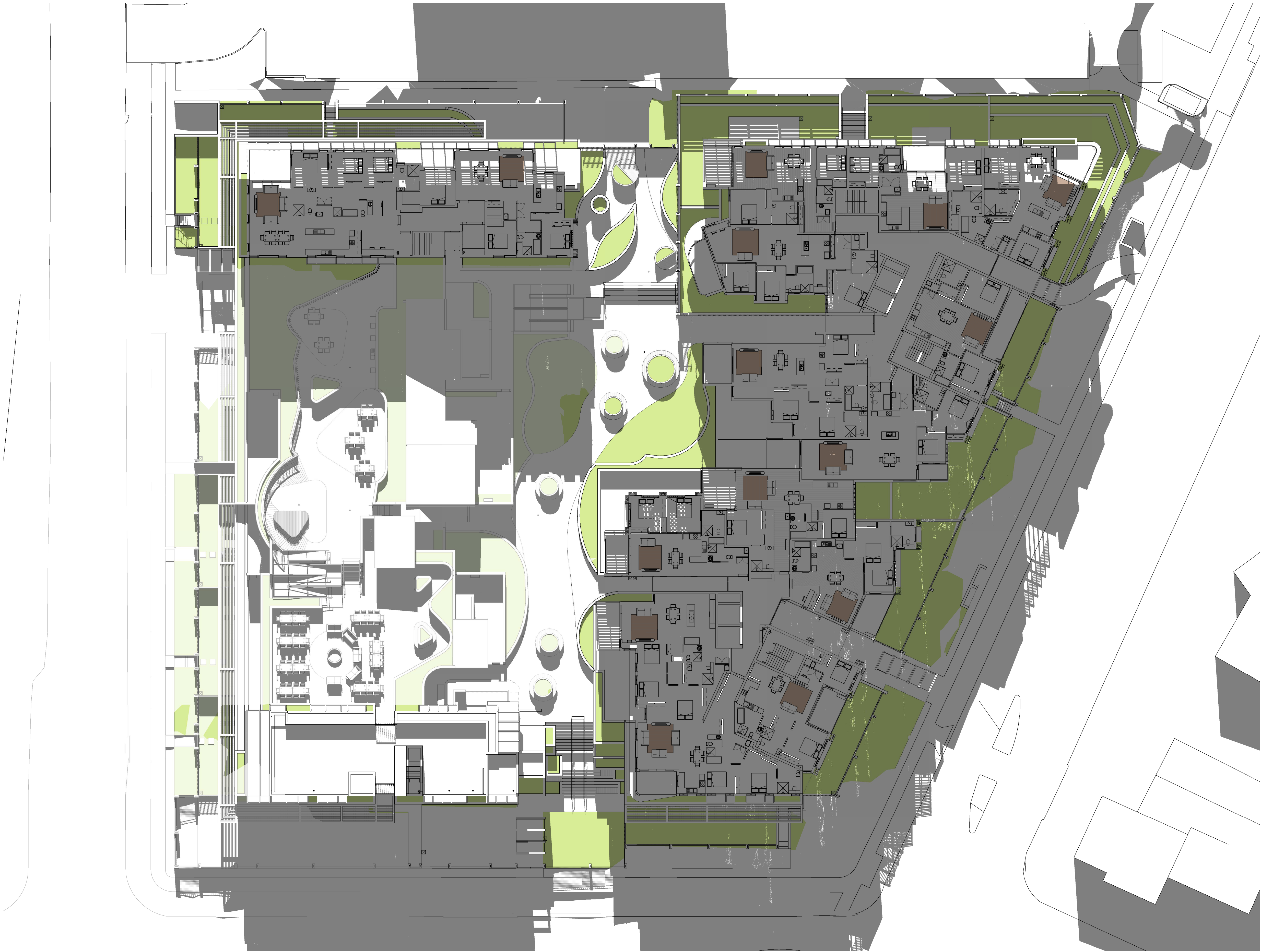
1 Internal Solar Access - Level 4 11am June 21
