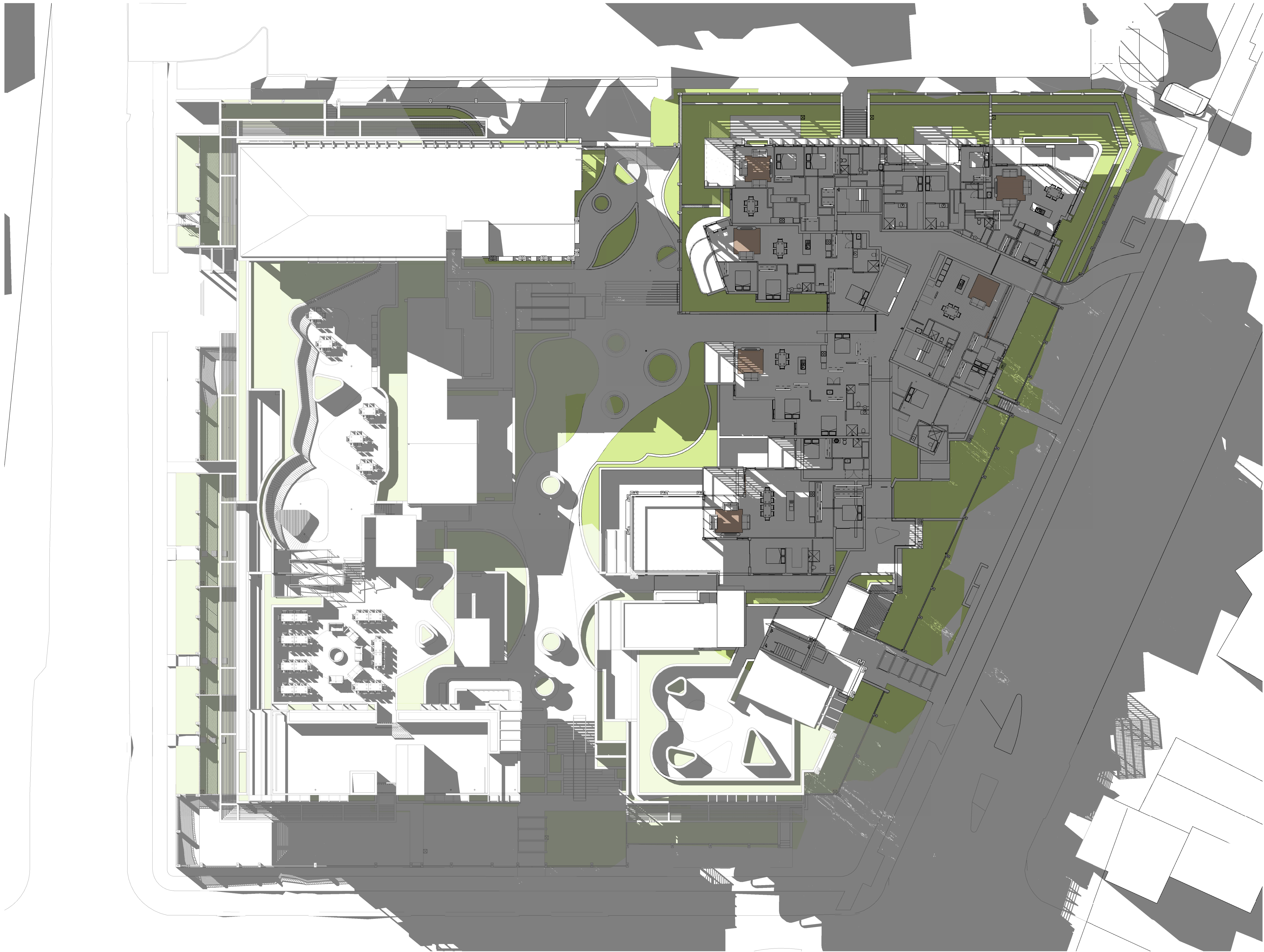
1 Internal Solar Access - Level 5 2pm June 21
