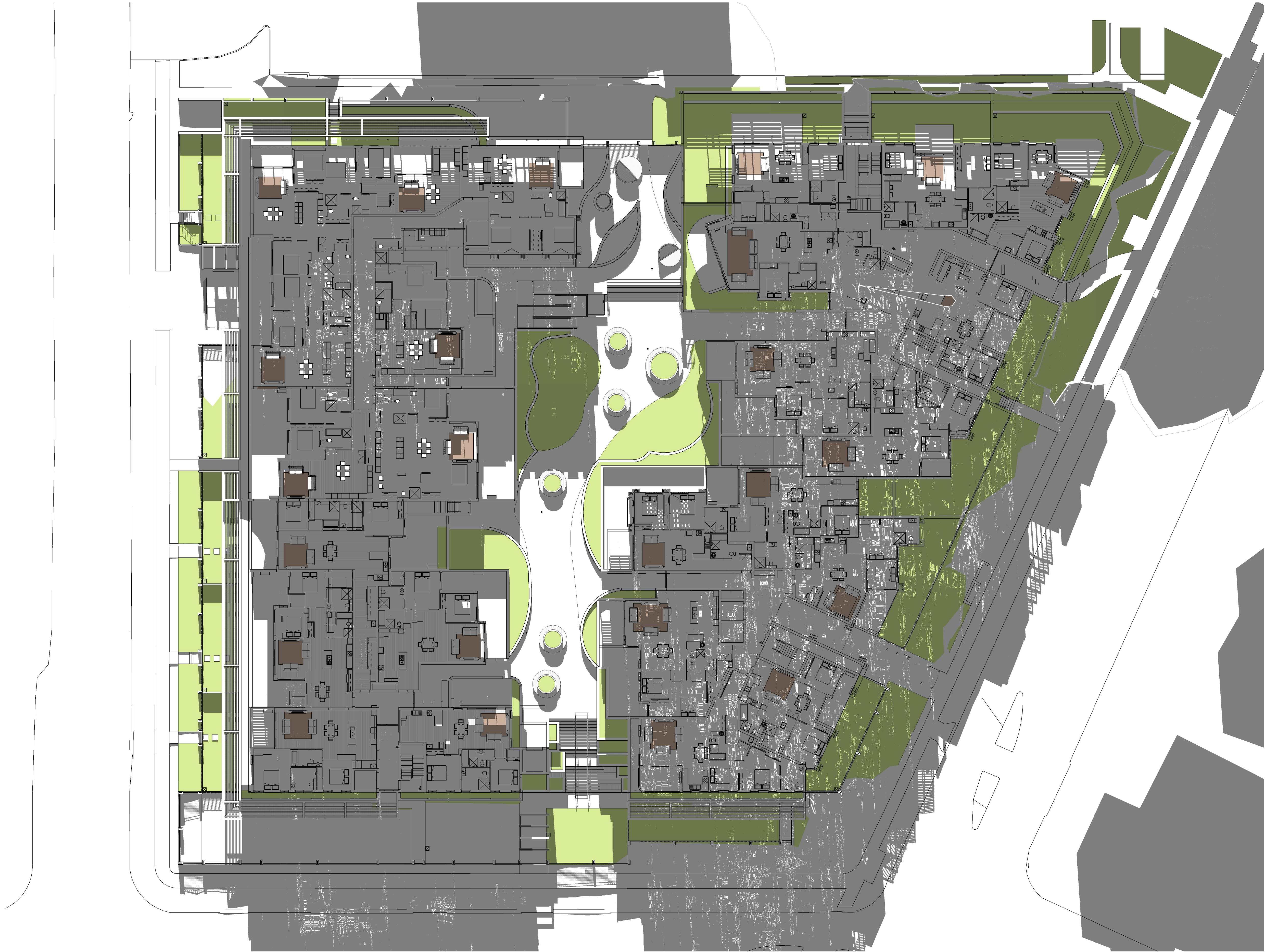
1 Internal Solar Access - Level 1 11am June 21
