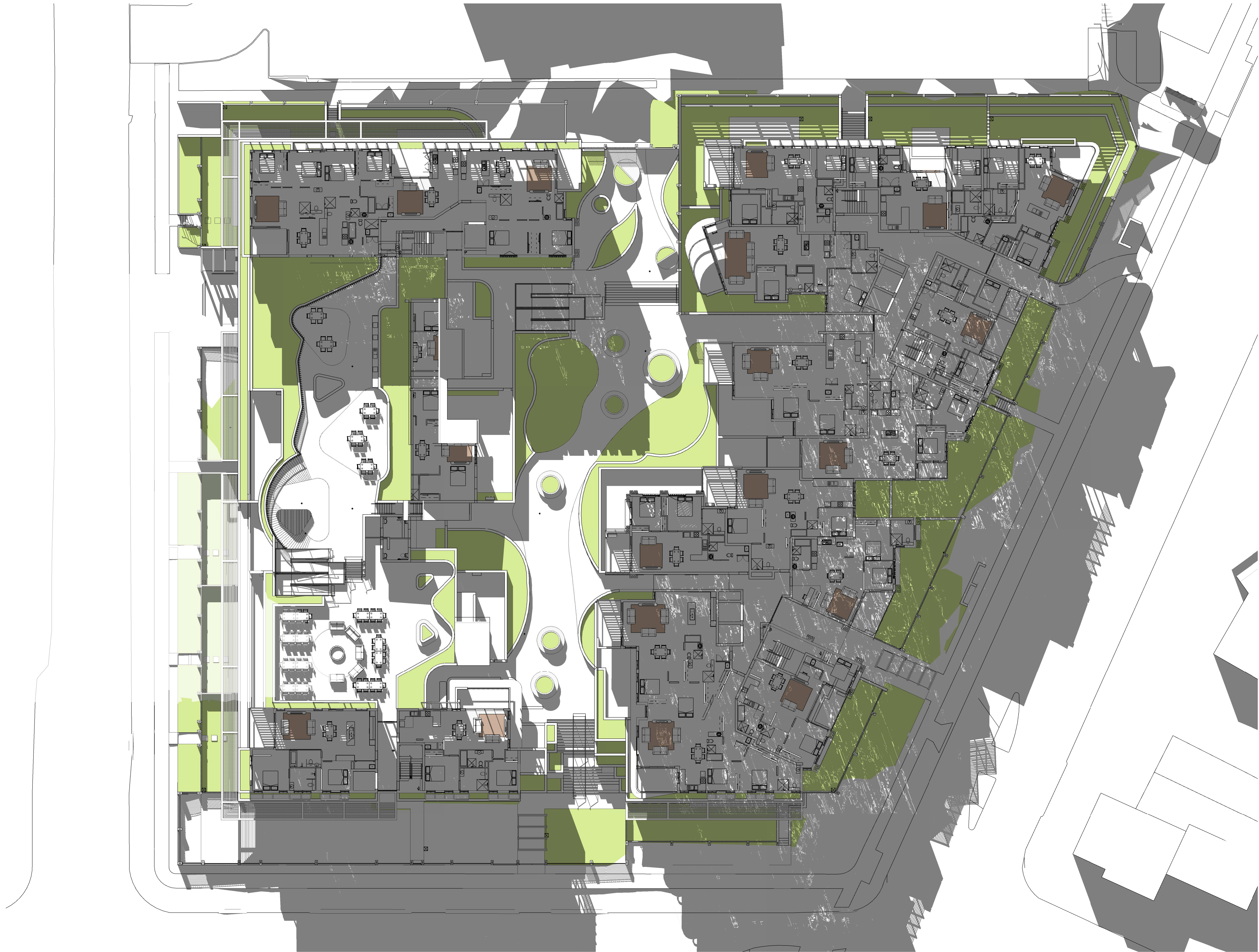
1 Internal Solar Access - Level 2 12pm June 21
