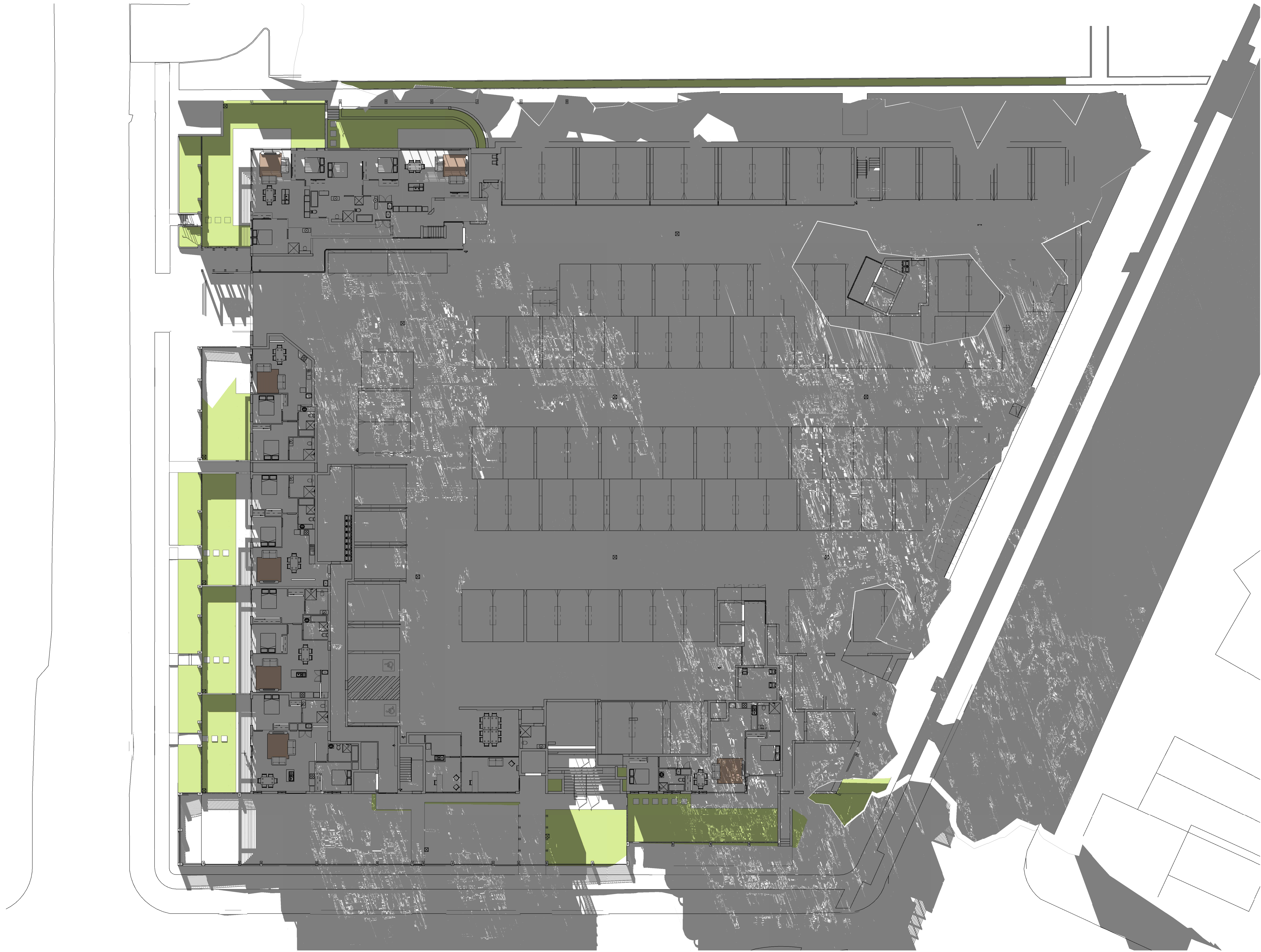
1 Internal Solar Access - Ground Floor 12pm June 21
